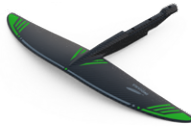
MB Front Wing Marlin XXS Proj. Area: 540 cm 2 Span: 635 mm | Aspect Ratio: 7.5 Art. 3566SQ
